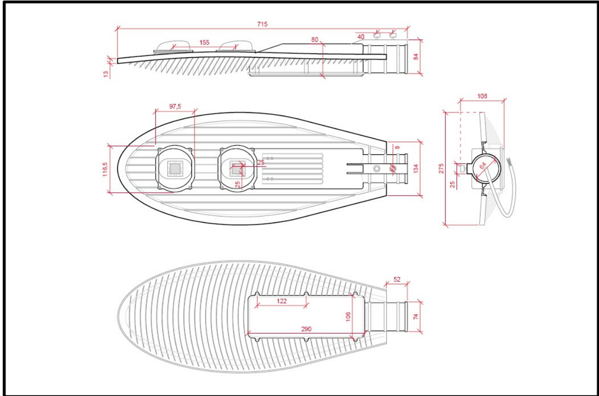
LED Street Light 120W 12000Lm 50.000H
